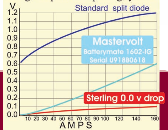
Voltage drop across splitting systems
